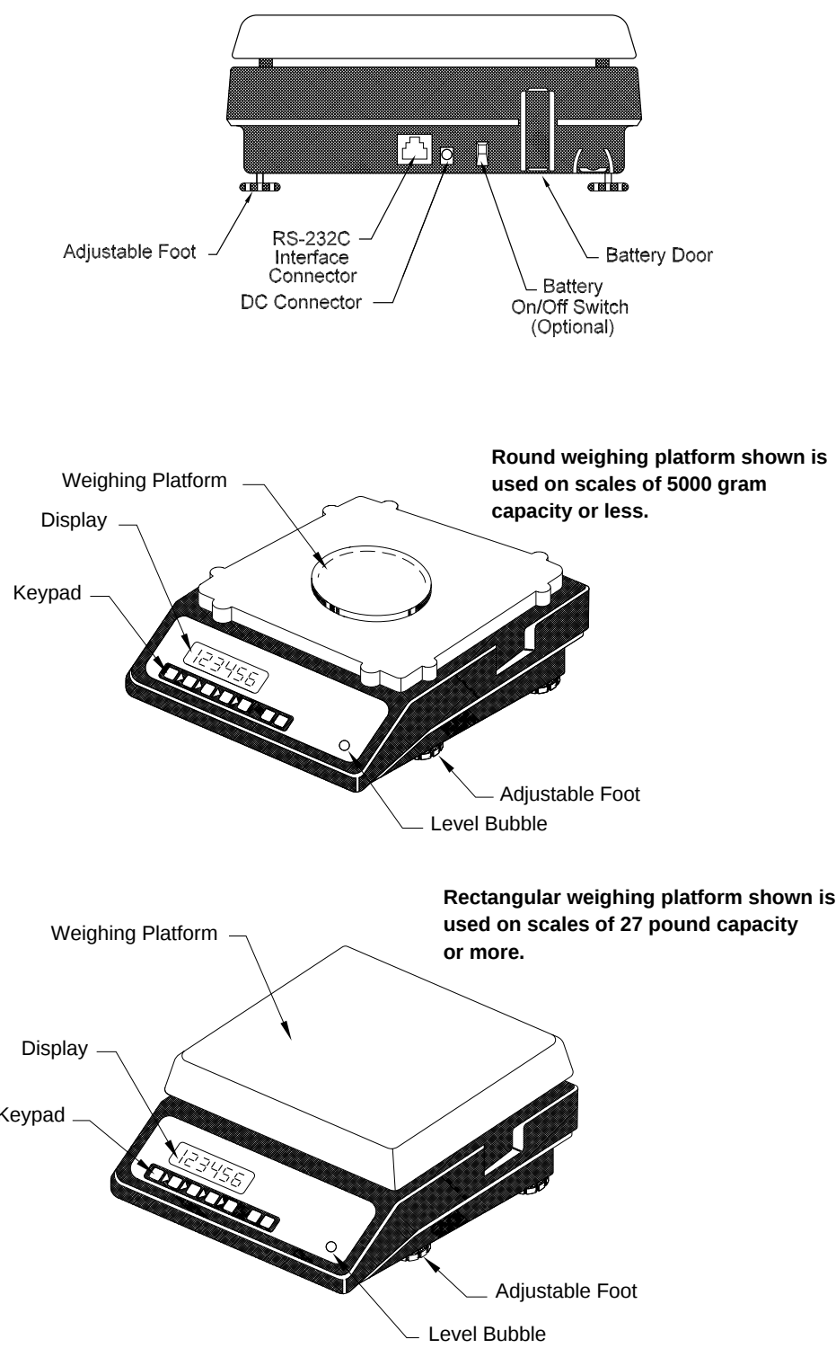
FIGURE 1. Components and features of the Setra Quick Count.
